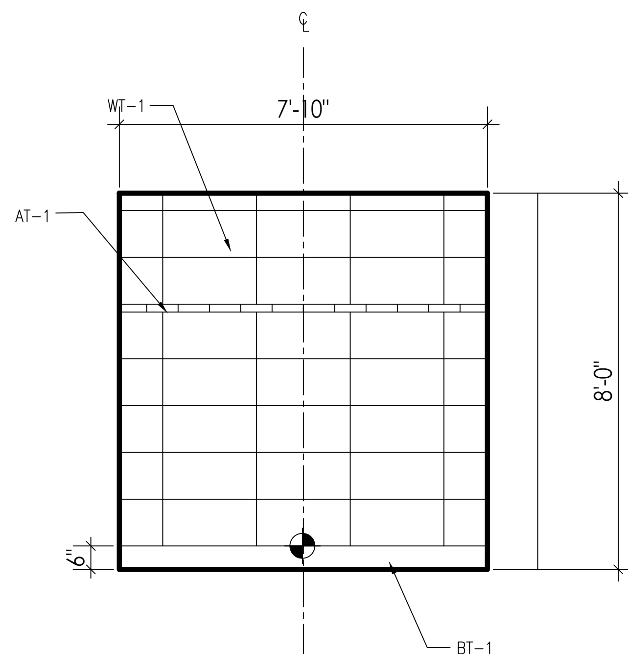
03 1/2"=1'-0" ELEVATIONS: 9TH FLOOR BATHROOMS
