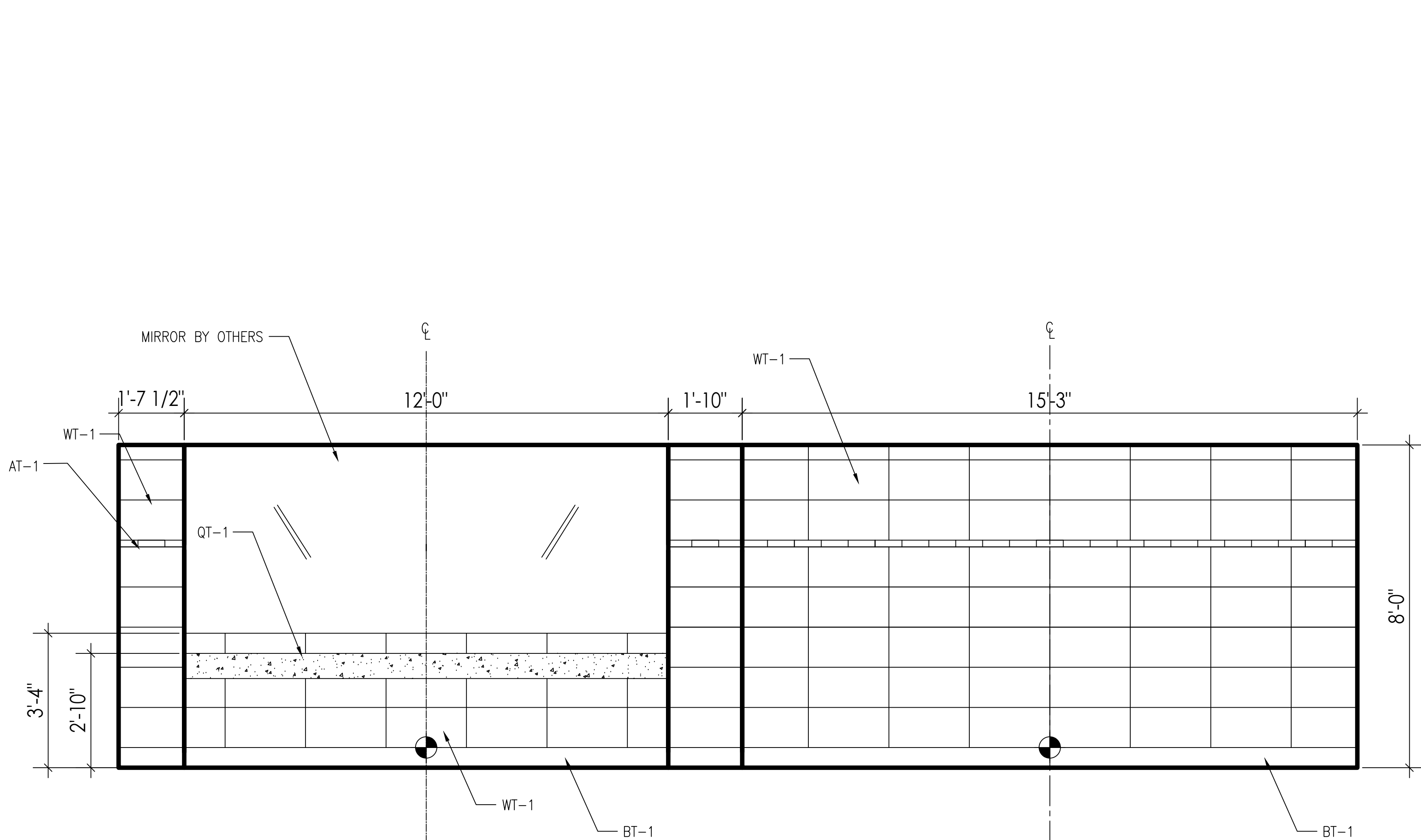
04 1/2"=1'-0" ELEVATIONS: 7TH FLOOR BATHROOMS
