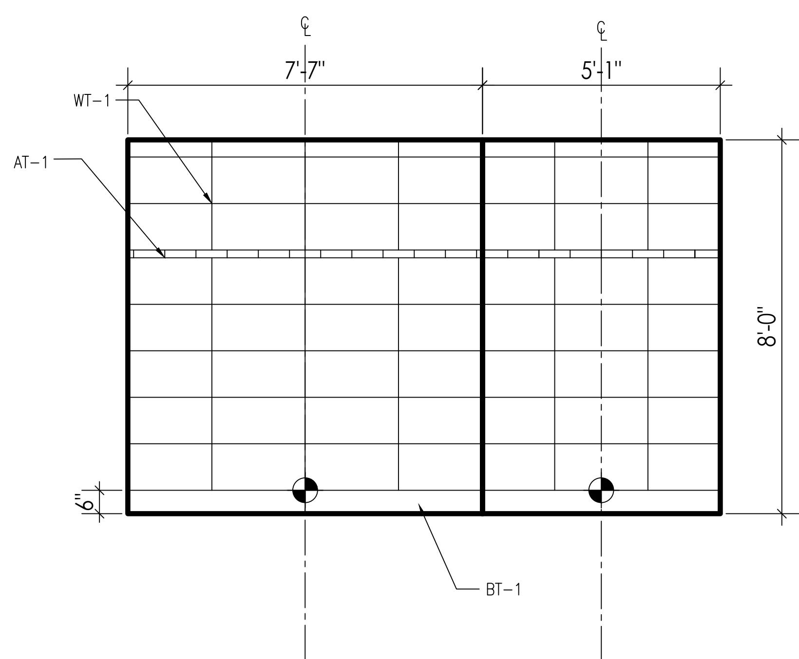
03 1/2"=1'-0" ELEVATIONS: 7TH FLOOR BATHROOMS
