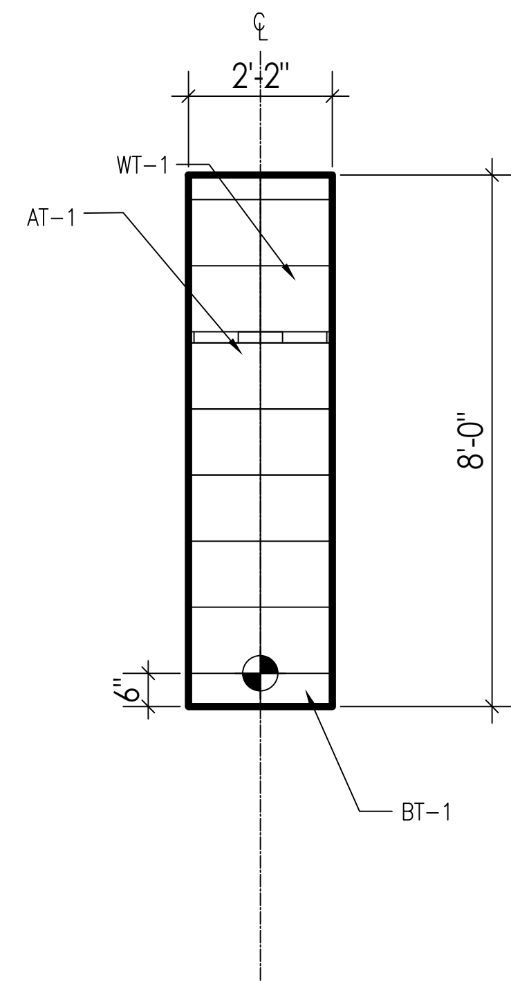
03 1/2"=1'-0" ELEVATIONS: 6TH FLOOR BATHROOMS
