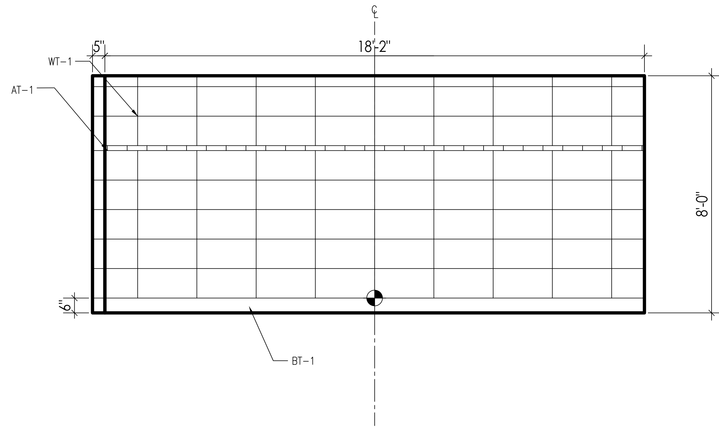
04 1/2"=1'-0" ELEVATIONS: 9TH FLOOR BATHROOMS
