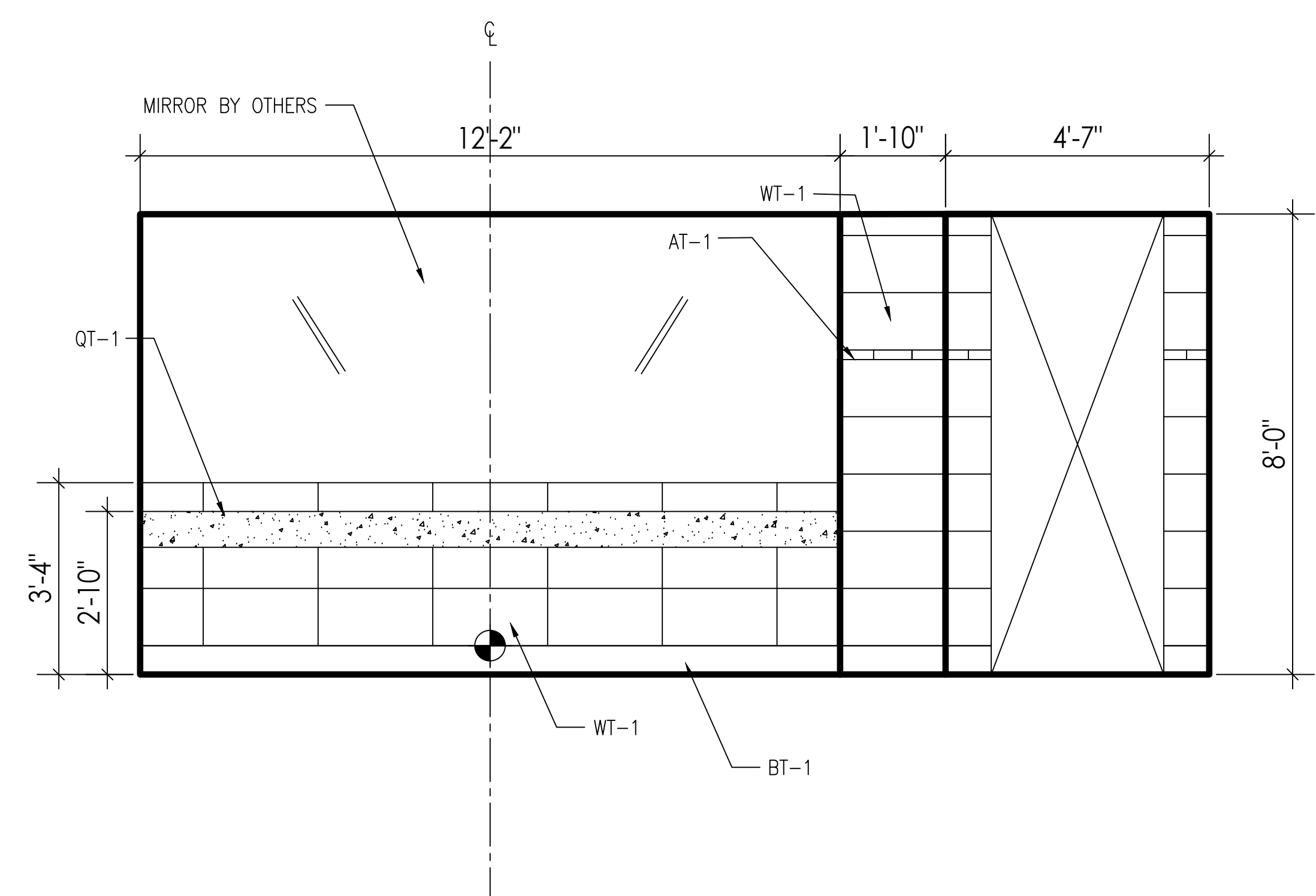
02 1/2"=1'-0" ELEVATIONS: 6TH FLOOR BATHROOMS
