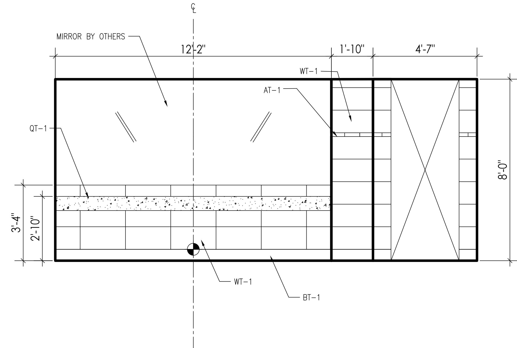
02 1/2"=1'-0" ELEVATIONS: 9TH FLOOR BATHROOMS
