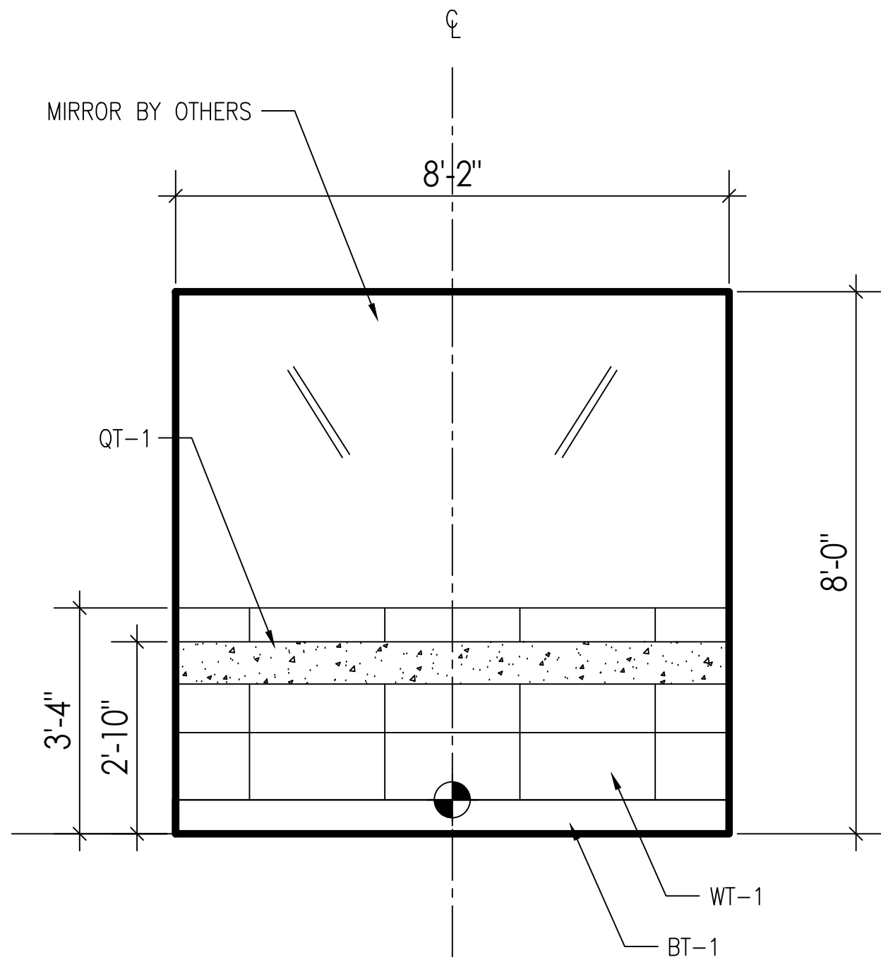
02 1/2"=1'-0" ELEVATIONS: 6TH FLOOR BATHROOMS
