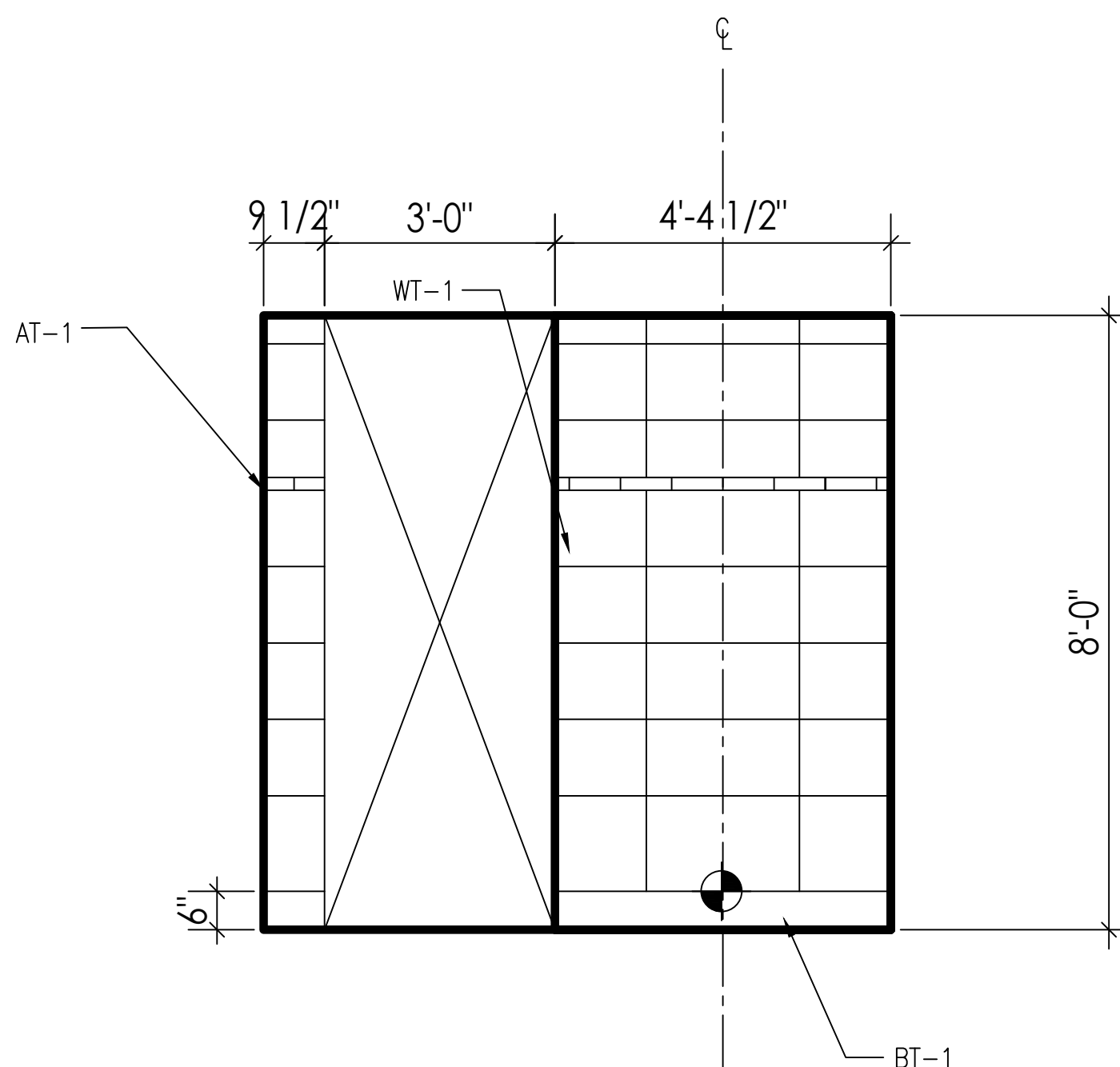
04 1/2"=1'-0" ELEVATIONS: 9TH FLOOR BATHROOMS
