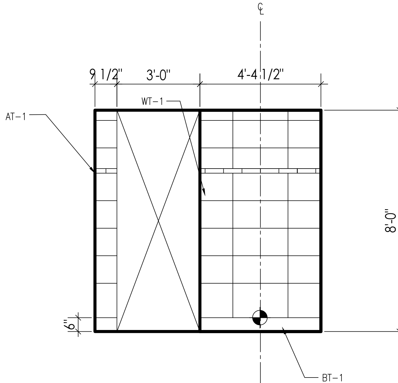
04 1/2"=1'-0" ELEVATIONS: 7TH FLOOR BATHROOMS
