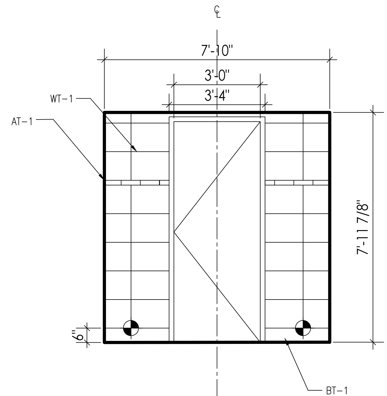
05 1/2"=1'-0" ELEVATIONS: 6TH FLOOR BATHROOMS
