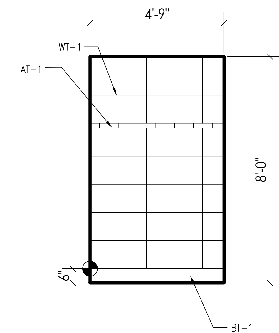
04 1/2"=1'-0" ELEVATIONS: 6TH FLOOR BATHROOMS
