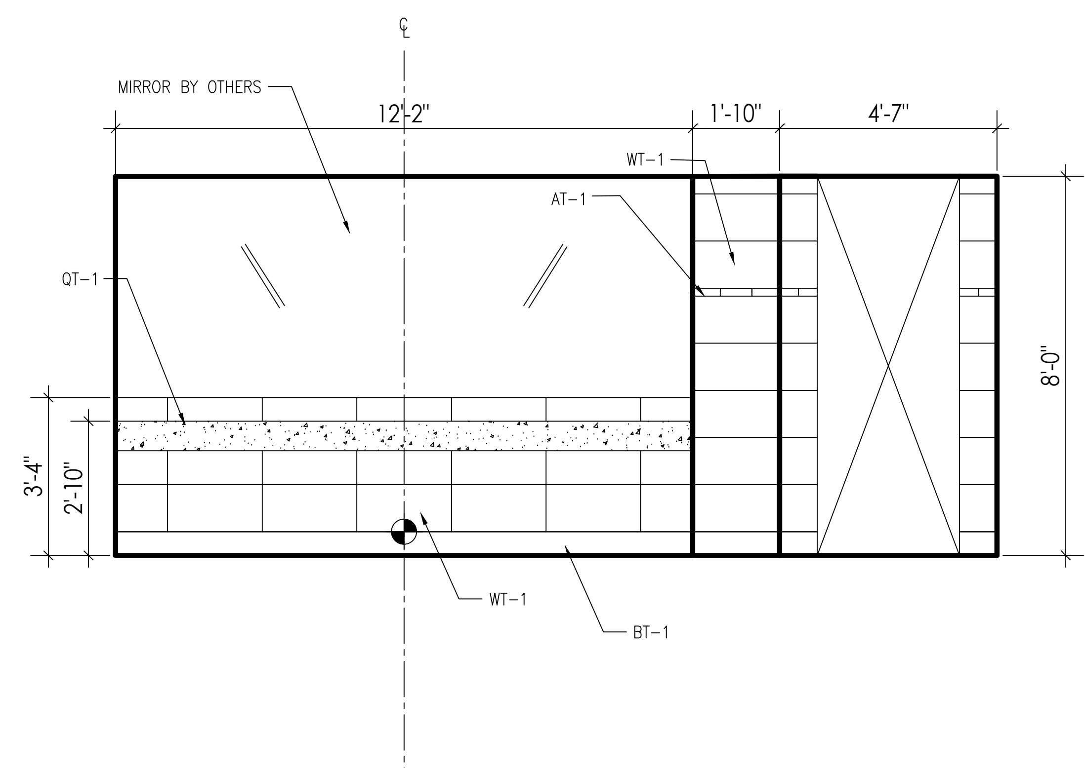
02 1/2"=1'-0" ELEVATIONS: 7TH FLOOR BATHROOMS
