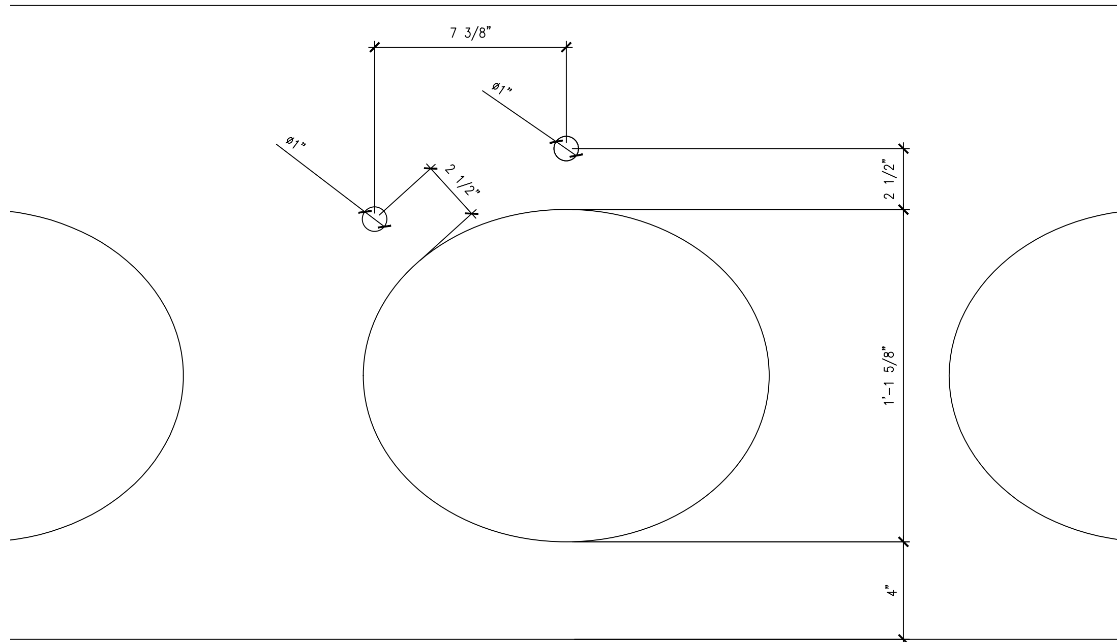
05 3/4"x1'-0" STONE COUNTERTOPS -7TH FLOOR MEN'S DETAIL VIEW
