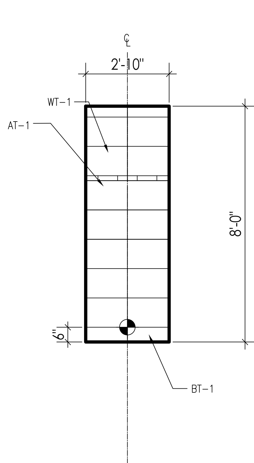
02 1/2"=1'-0" ELEVATIONS: 6TH FLOOR BATHROOMS
