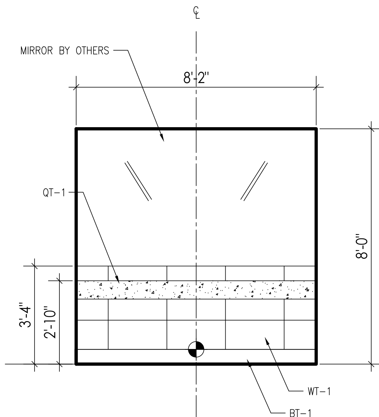
02 1/2"=1'-0" ELEVATIONS: 9TH FLOOR BATHROOMS
