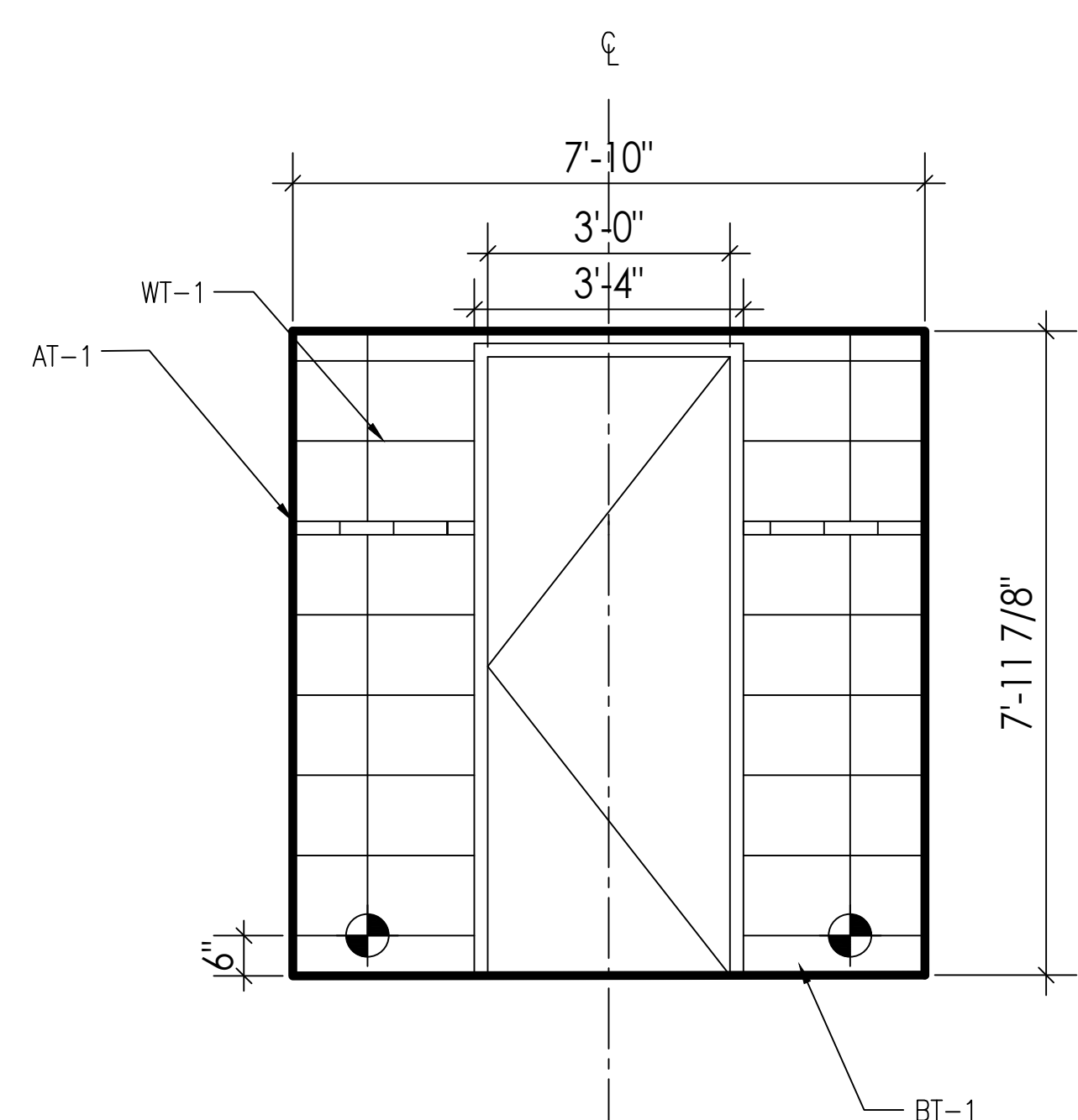
05 1/2"=1'-0" ELEVATIONS: 9TH FLOOR BATHROOMS
