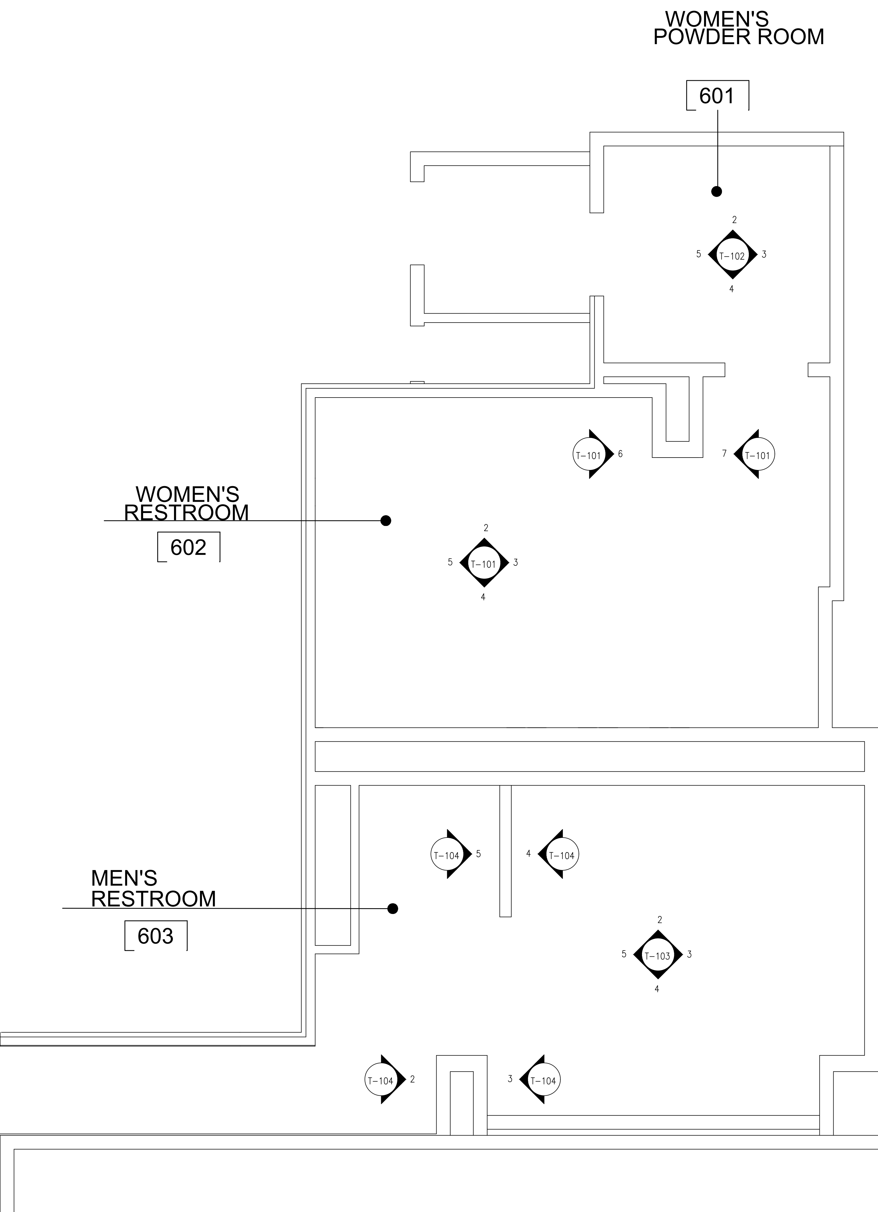
01 1/2"=1'-0" PLAN #2: 6TH FLOOR BATHROOMS
