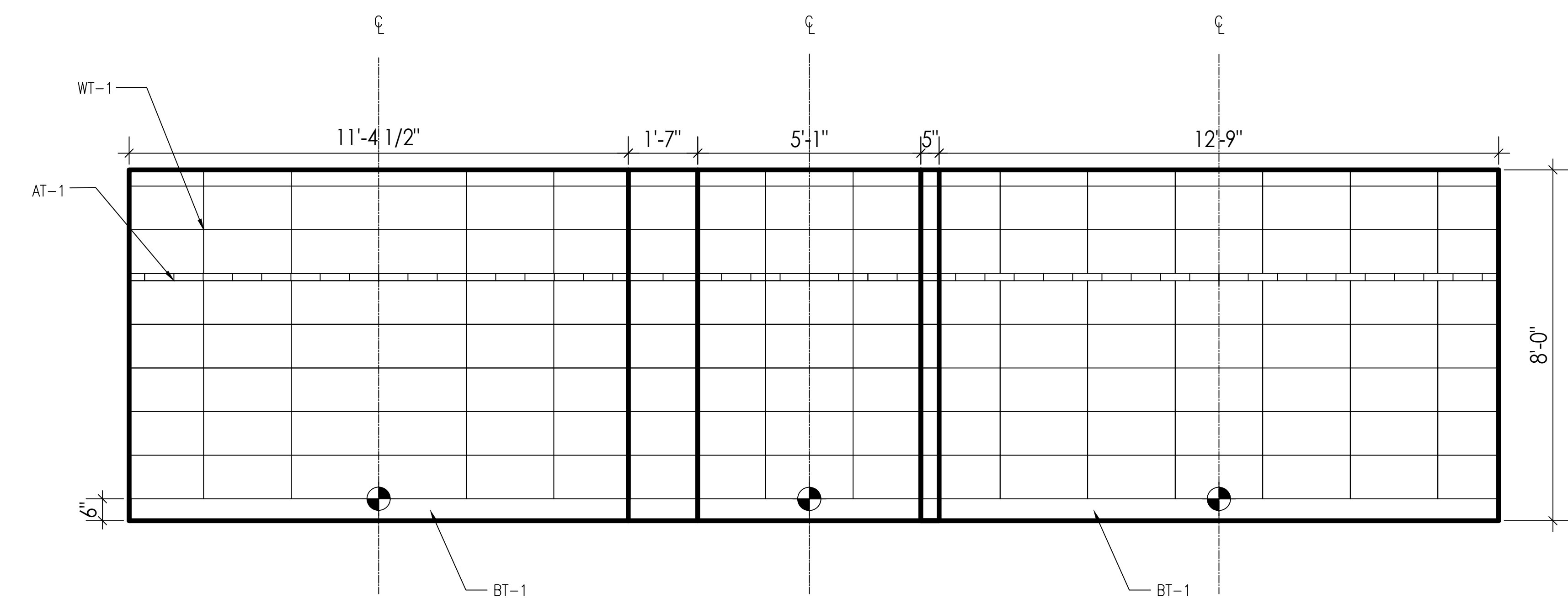
02 1/2"=1'-0" ELEVATIONS: 7TH FLOOR BATHROOMS
