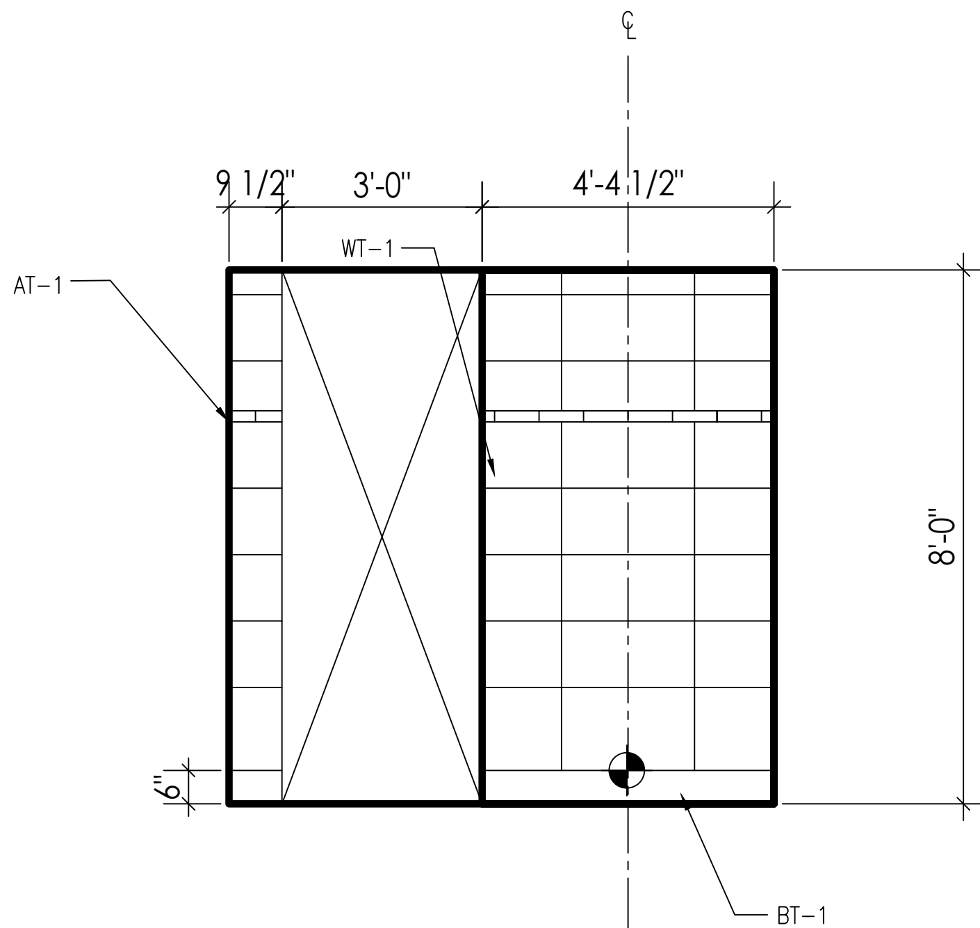
04 1/2"=1'-0" ELEVATIONS: 6TH FLOOR BATHROOMS
