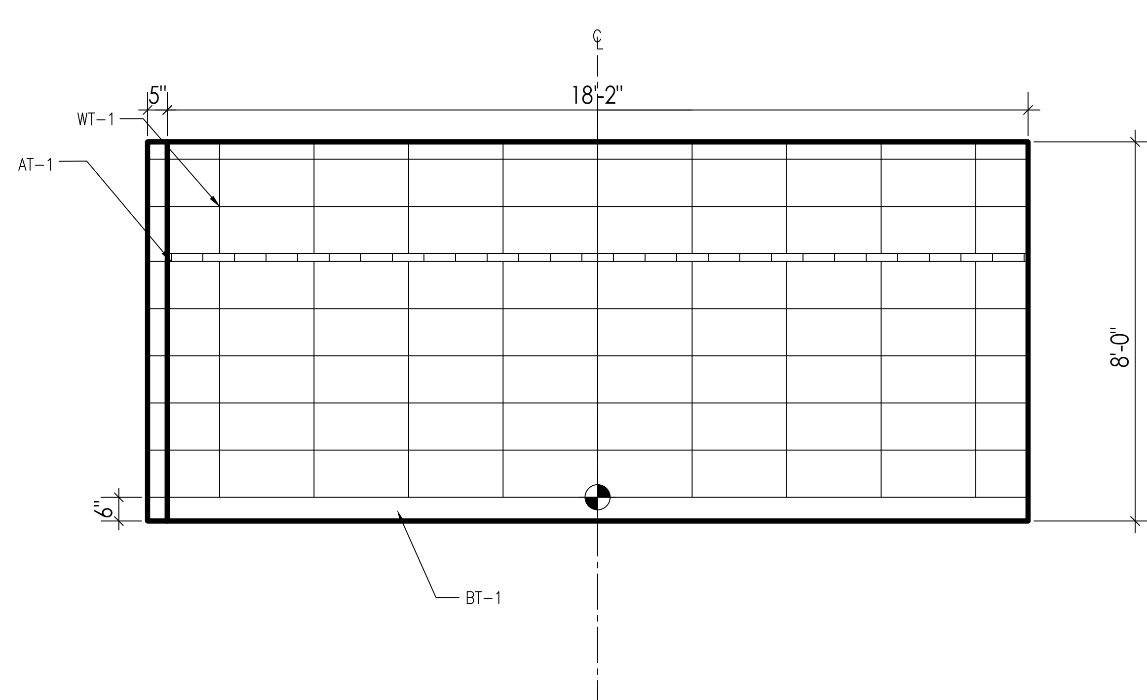
04 1/2"=1'-0" ELEVATIONS: 7TH FLOOR BATHROOMS
