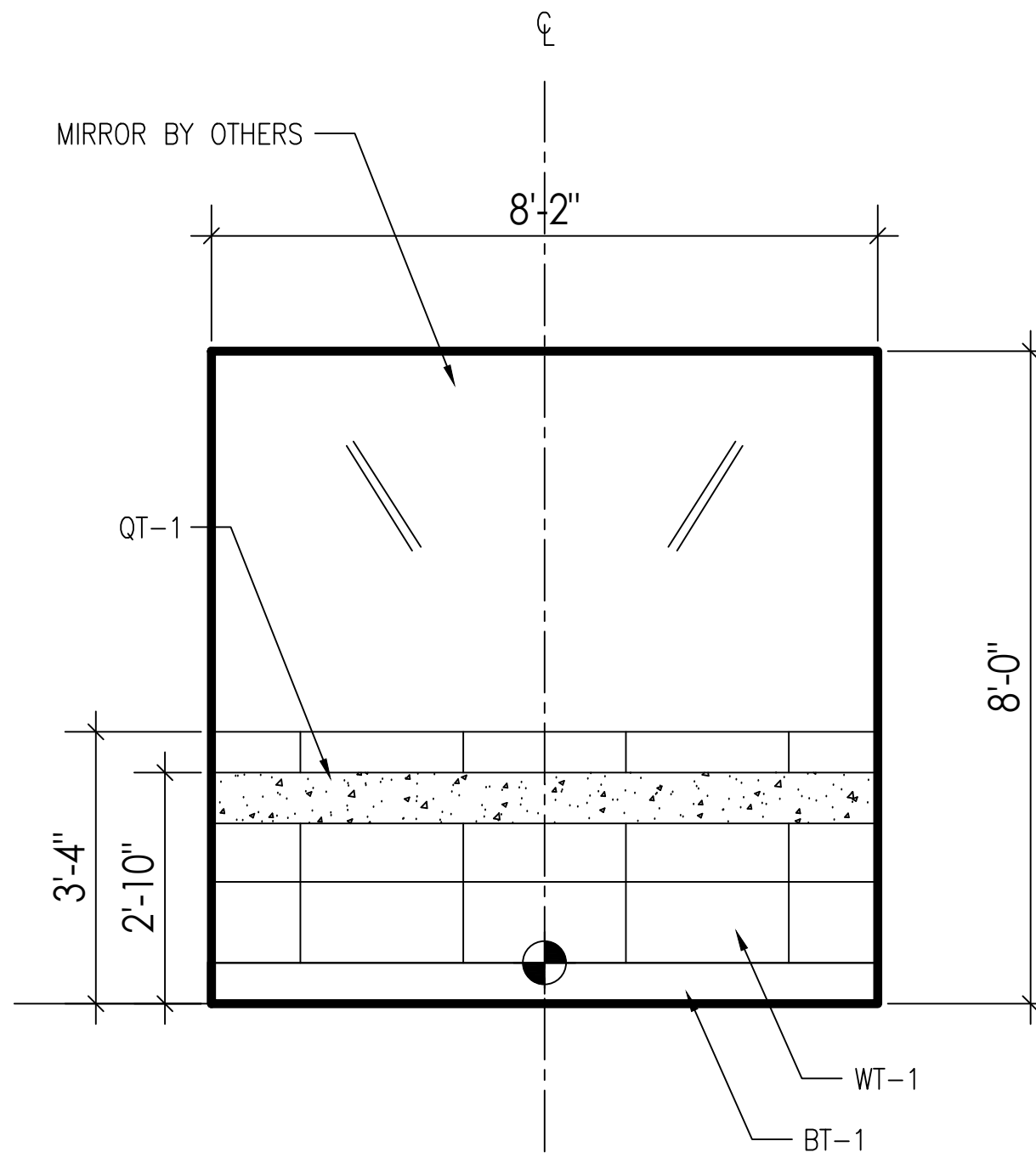
02 1/2"=1'-0" ELEVATIONS: 7TH FLOOR BATHROOMS
