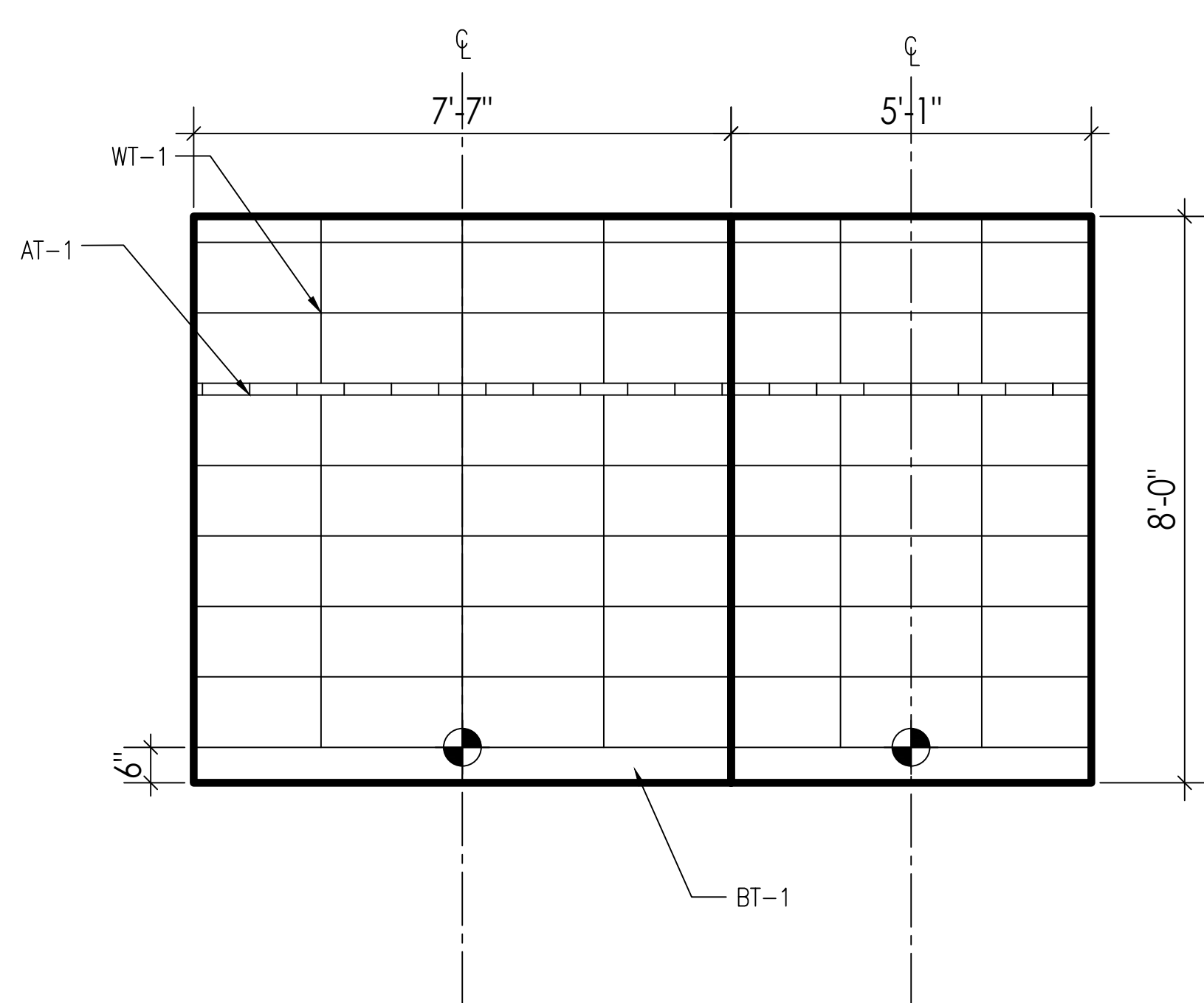
03 1/2"=1'-0" ELEVATIONS: 6TH FLOOR BATHROOMS
