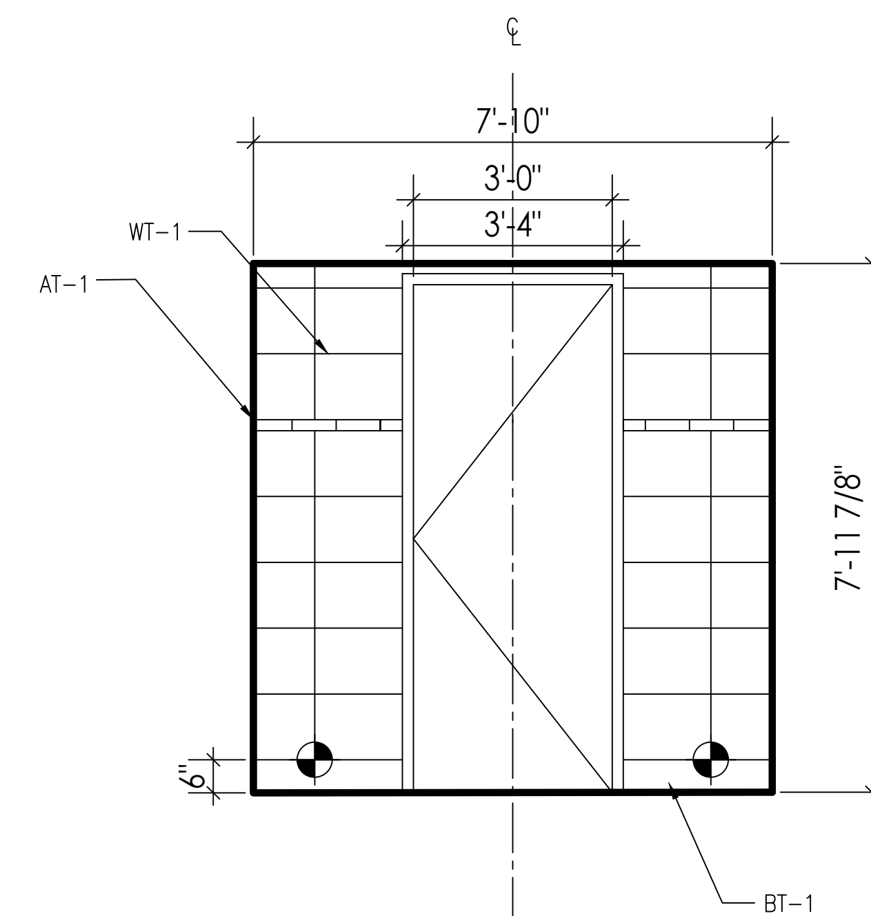
05 1/2"=1'-0" ELEVATIONS: 7TH FLOOR BATHROOMS
