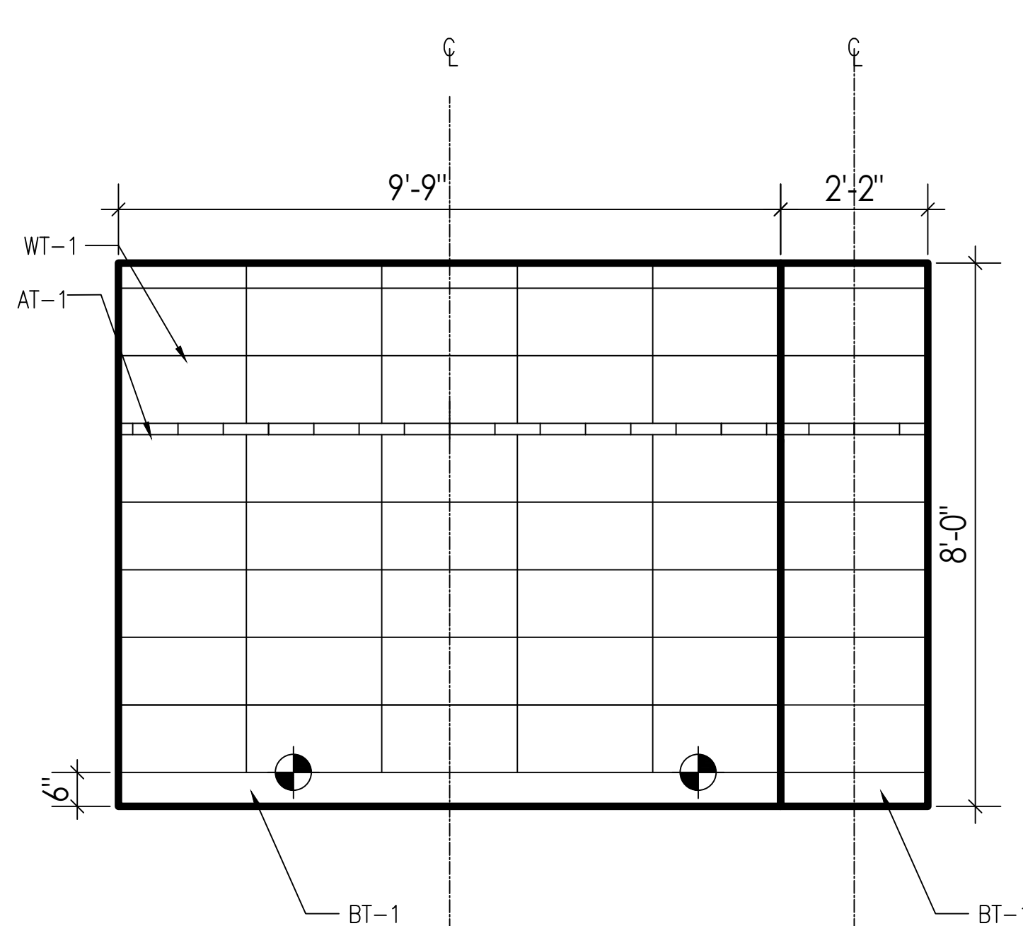
03 1/2"=1'-0" ELEVATIONS: 7TH FLOOR BATHROOMS
