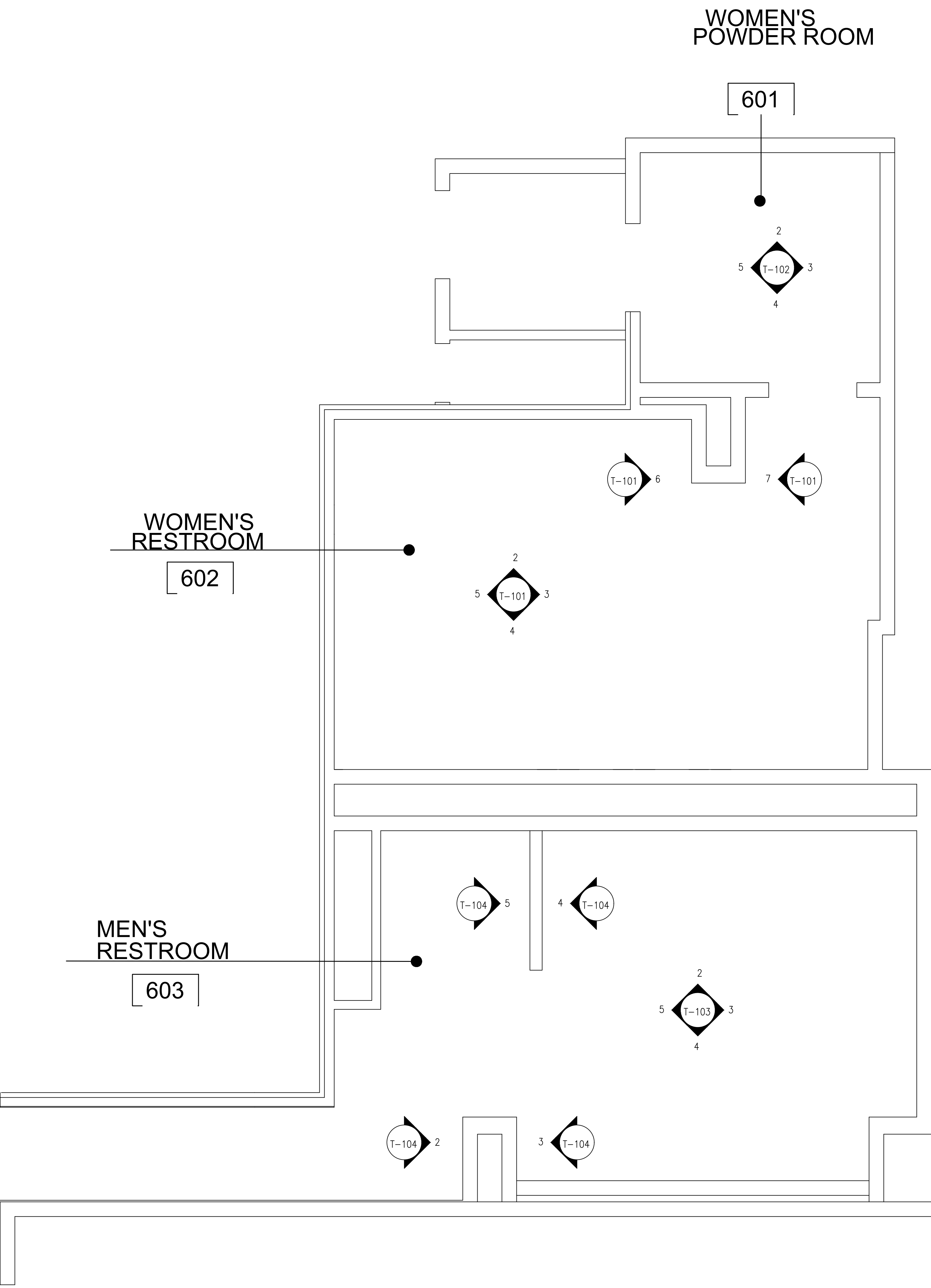
01 1/2"=1'-0" PLAN: 6TH FLOOR SINGLE BATHROOM
